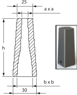
Anahtar adaptörü/ Key Adaptor
